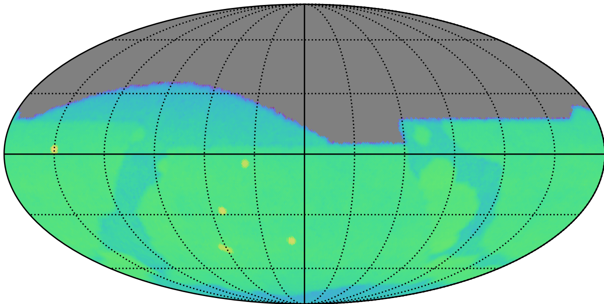
weather_cloudso16v3.4_10yrs g: CoaddM5
