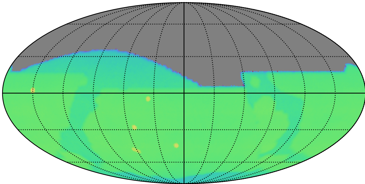
weather_cloudso16v3.4_10yrs : CoaddM5
