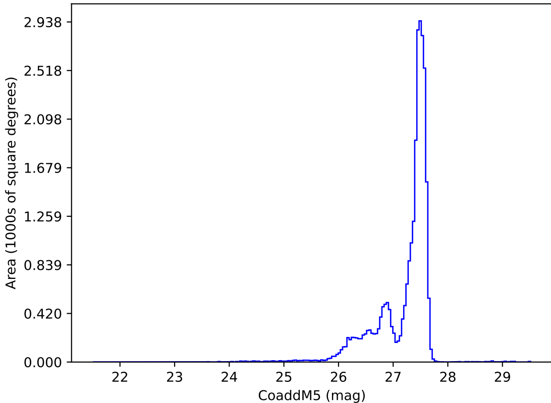
weather_cloudso16v3.4_10yrs : CoaddM5
