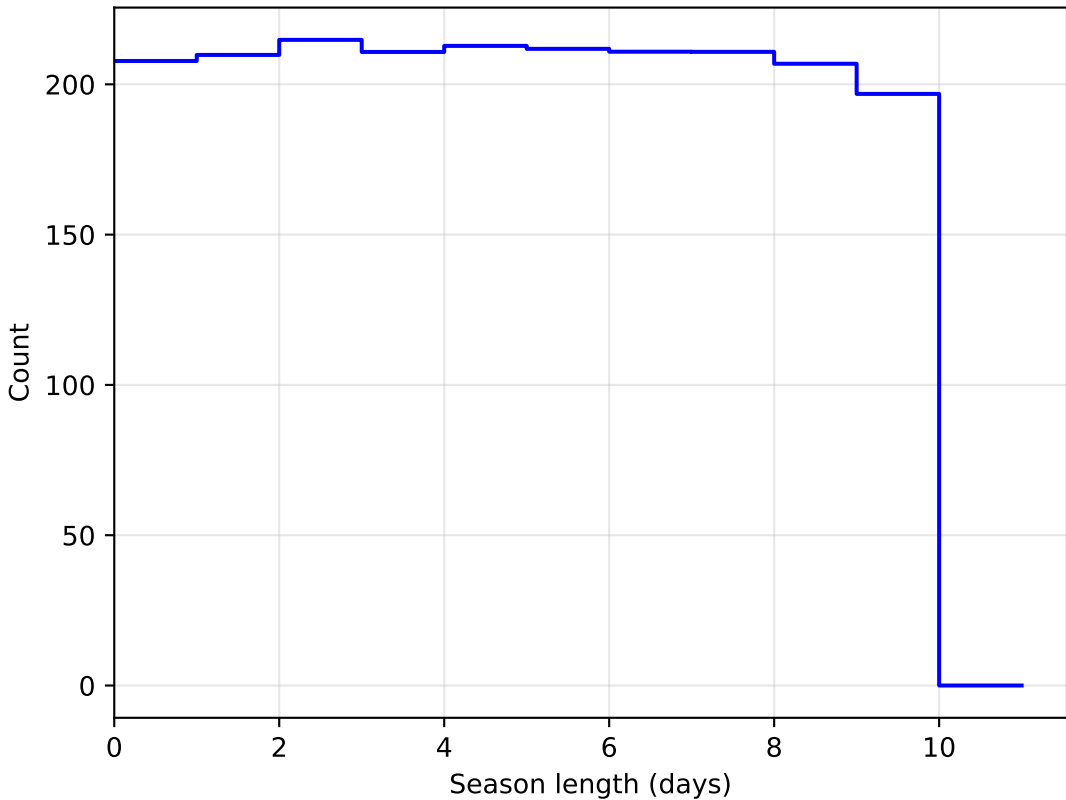
weather_cloudso16v3.4_10yrs DD:EDFS all bands: SeasonLength
