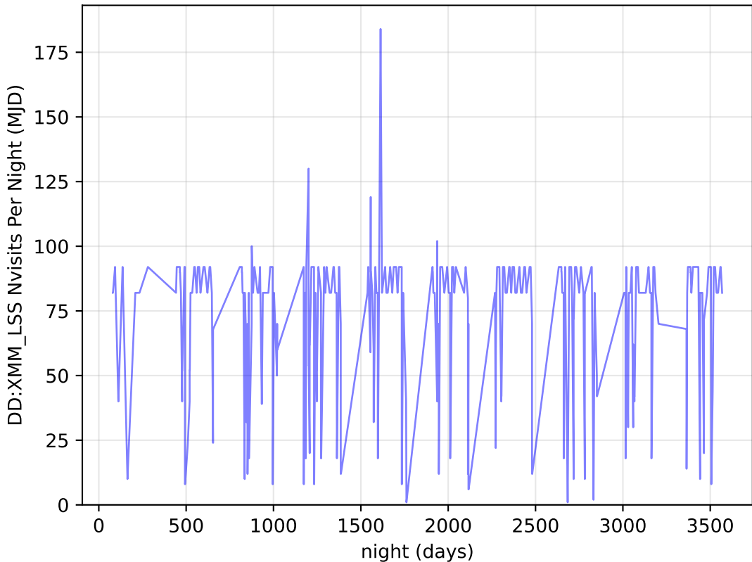
weather_cloudso16v3.4_10yrs all bands: DD:XMM_LSS Nvisits Per Night
