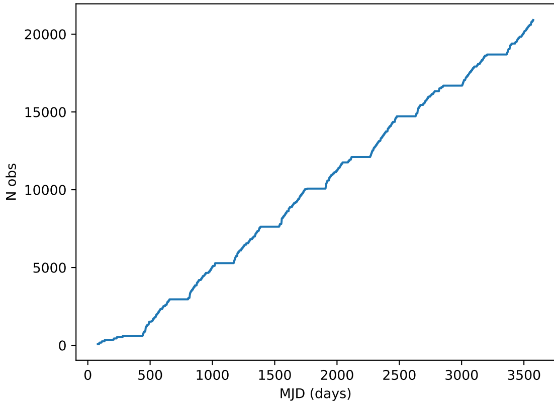
weather_cloudso16v3.4_10yrs all bands: DD:XMM_LSS Cumulative NVisits
