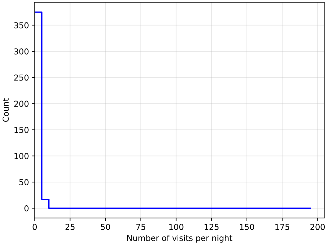
weather_cloudso16v3.4_10yrs all bands: DD:WFD NVisitsPerNight
