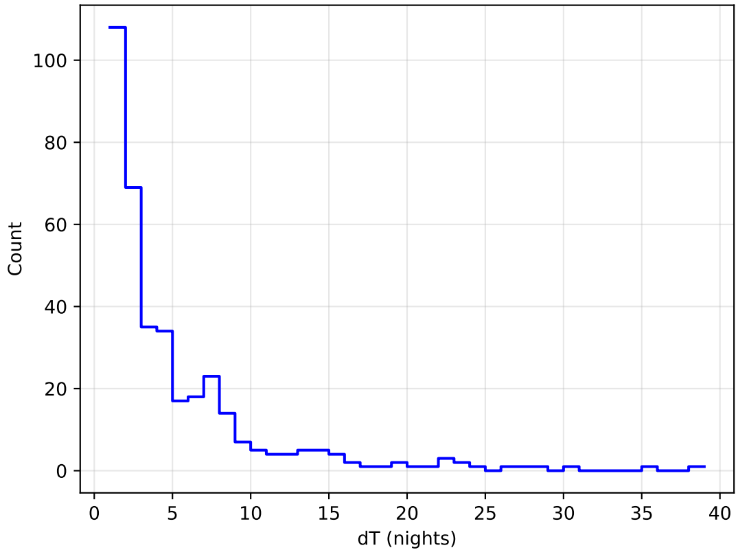
weather_cloudso16v3.4_10yrs all bands: DD:WFD Delta Nights Histogram
