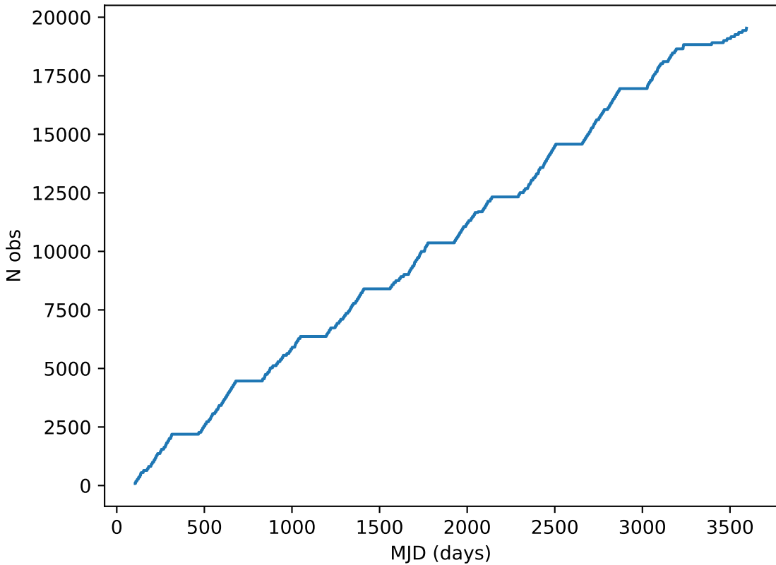
weather_cloudso16v3.4_10yrs all bands: DD:EDFS Cumulative NVisits
