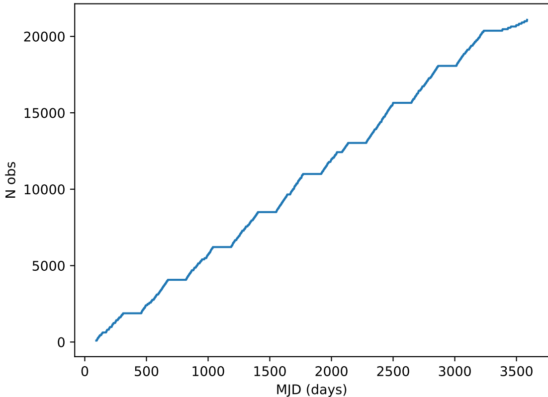
weather_cloudso16v3.4_10yrs all bands: DD:ECDFS Cumulative NVisits
