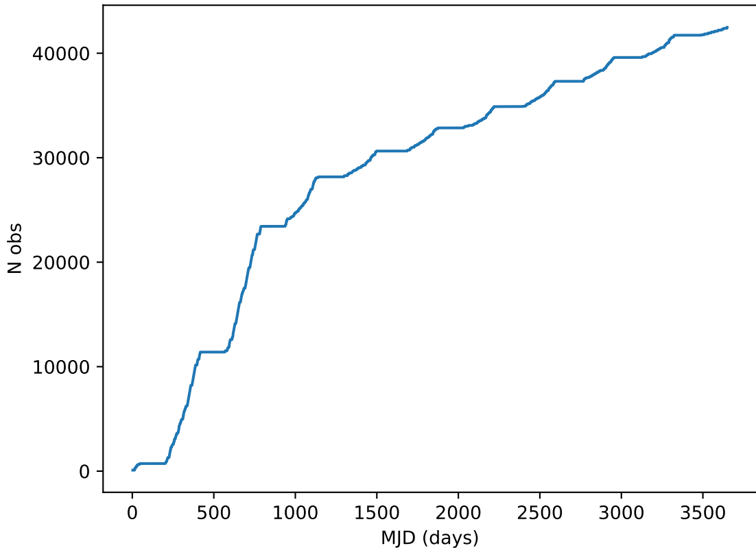
weather_cloudso16v3.4_10yrs all bands: DD:COSMOS Cumulative NVisits
