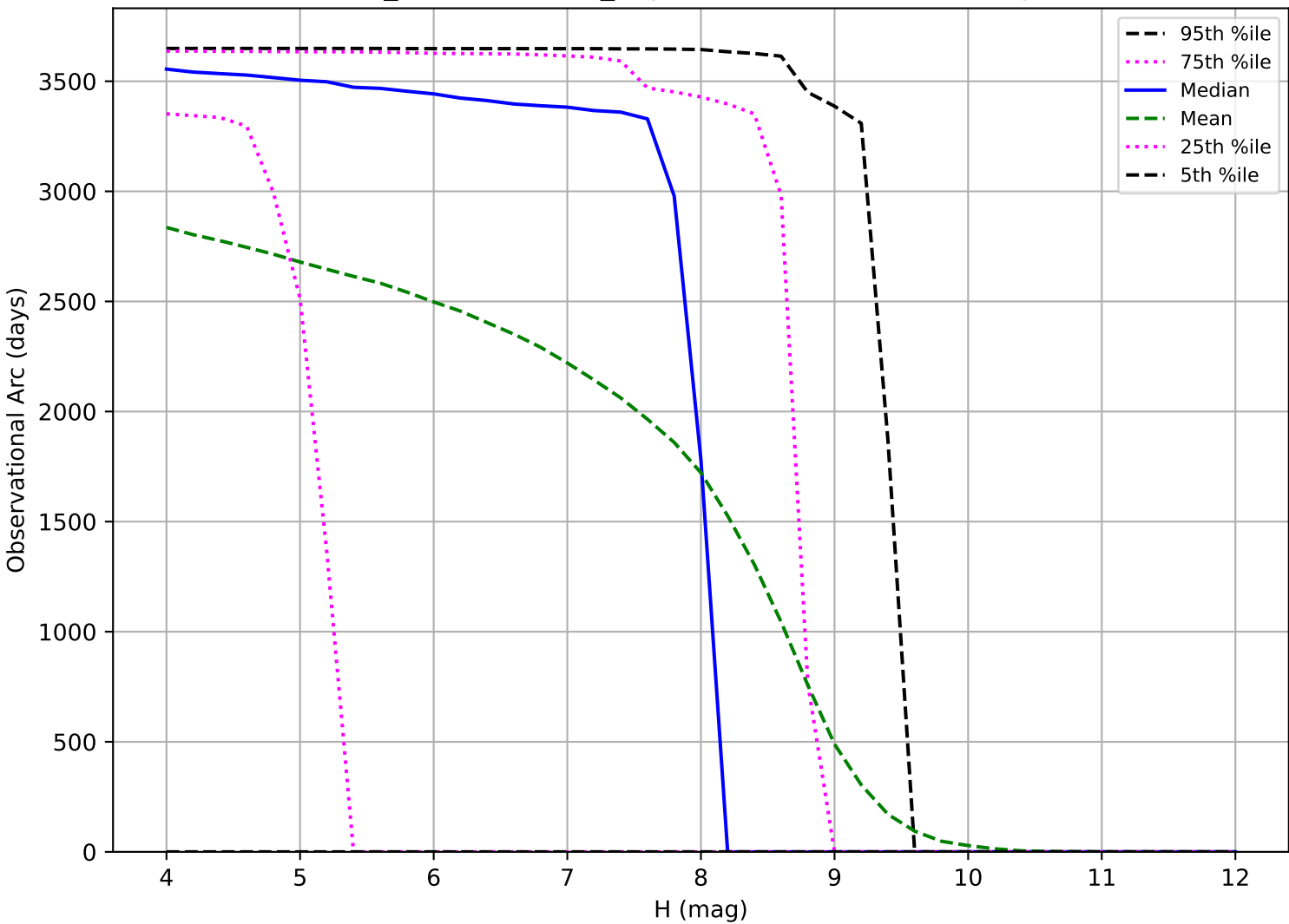
weather_cloudso14v3.4_10yrs: Observational Arc Length TNO
