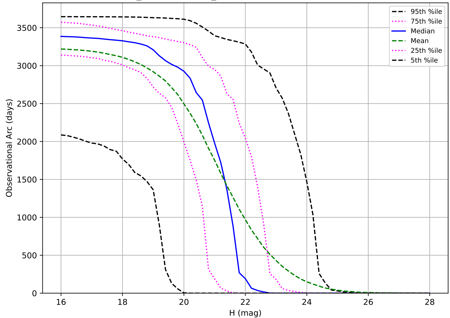
weather_cloudso14v3.4_10yrs: Observational Arc Length PHA
