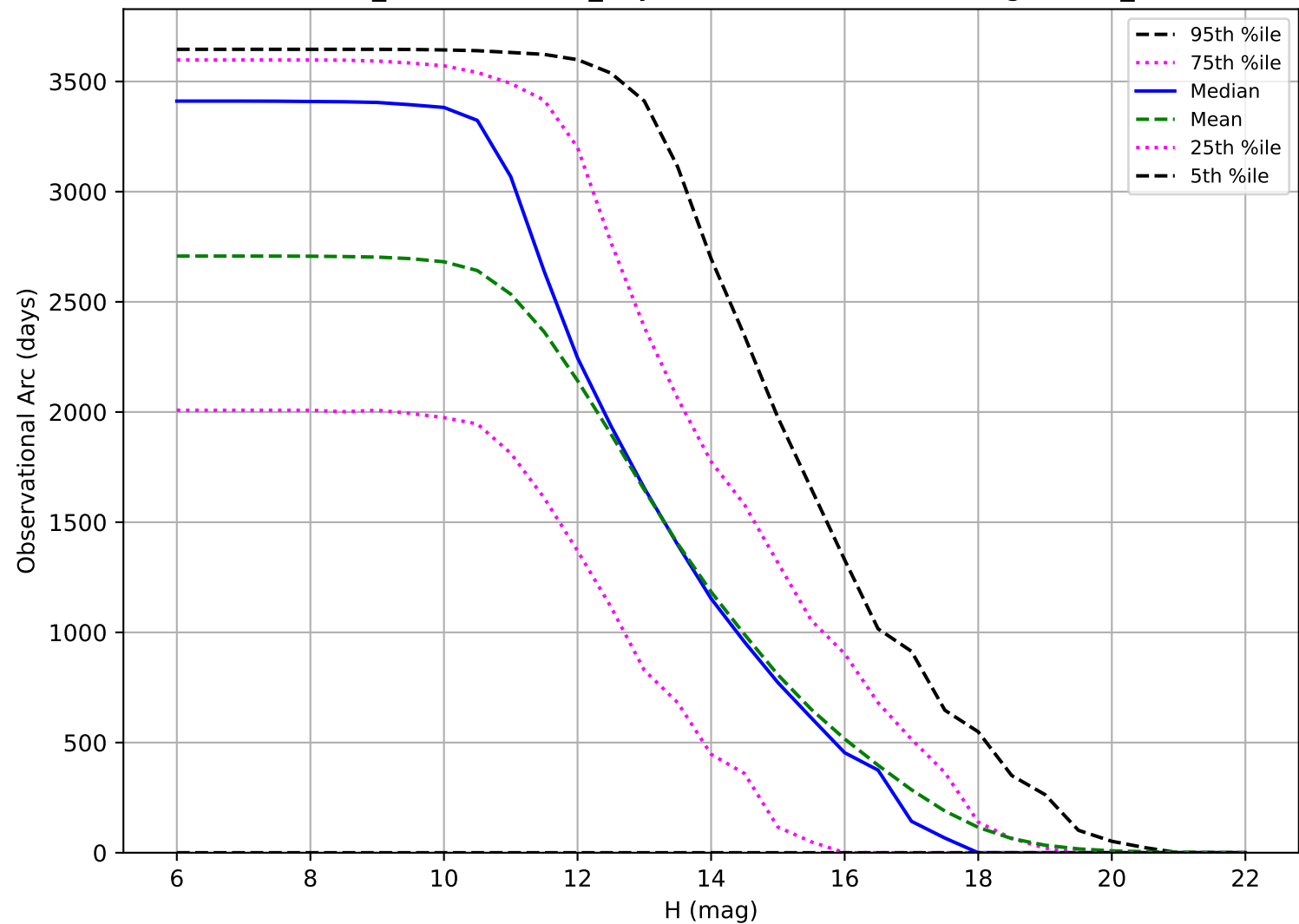
weather_cloudso14v3.4_10yrs: Observational Arc Length OCC_r5
