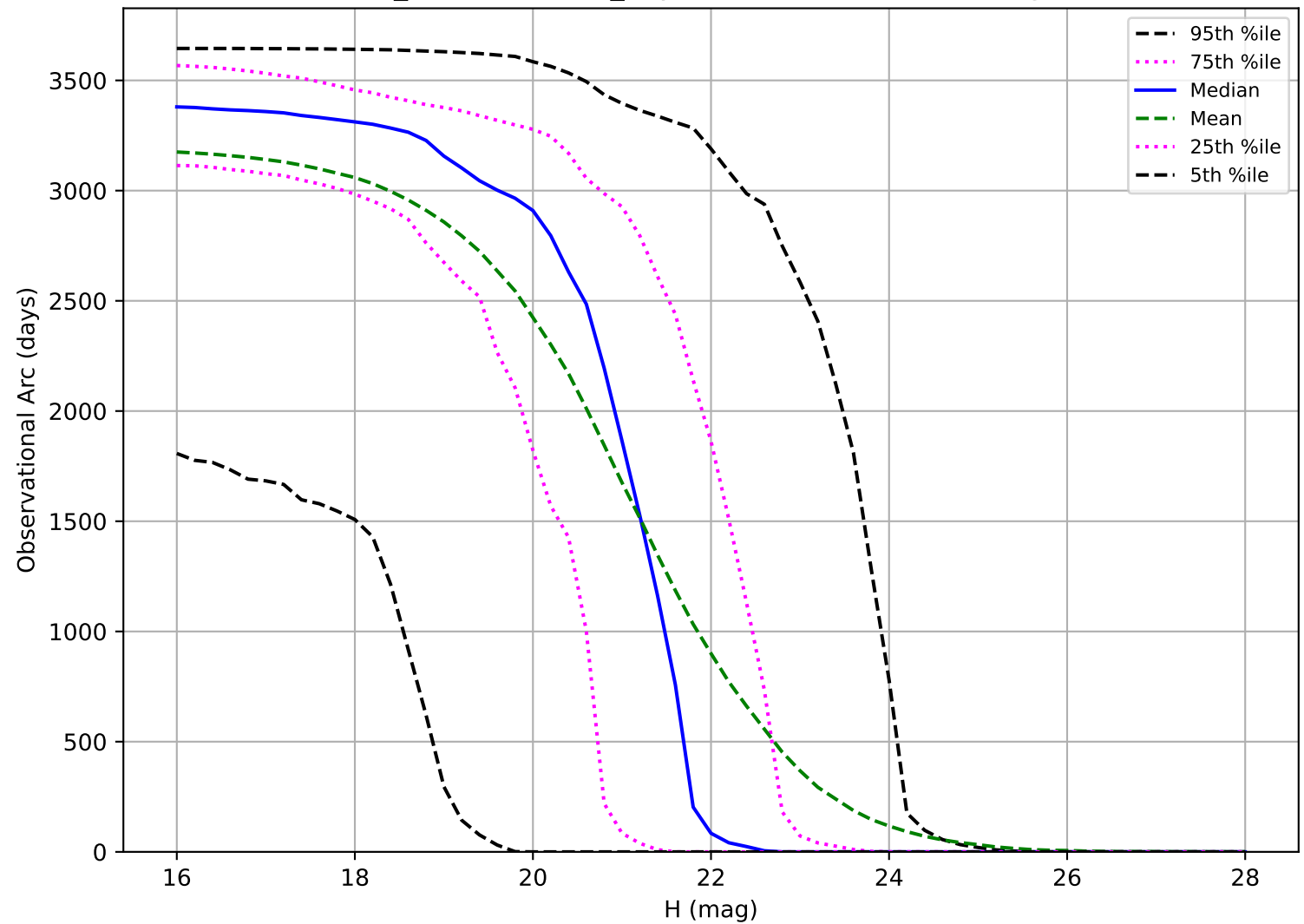
weather_cloudso14v3.4_10yrs: Observational Arc Length NEO
