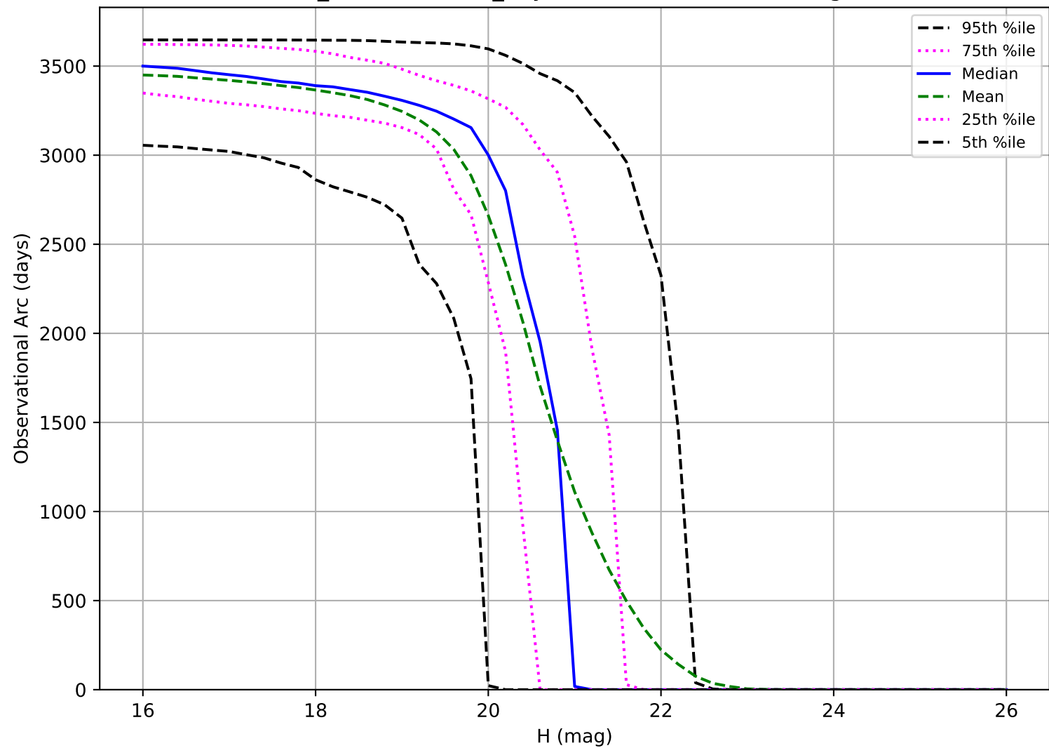
weather_cloudso14v3.4_10yrs: Observational Arc Length MBA
