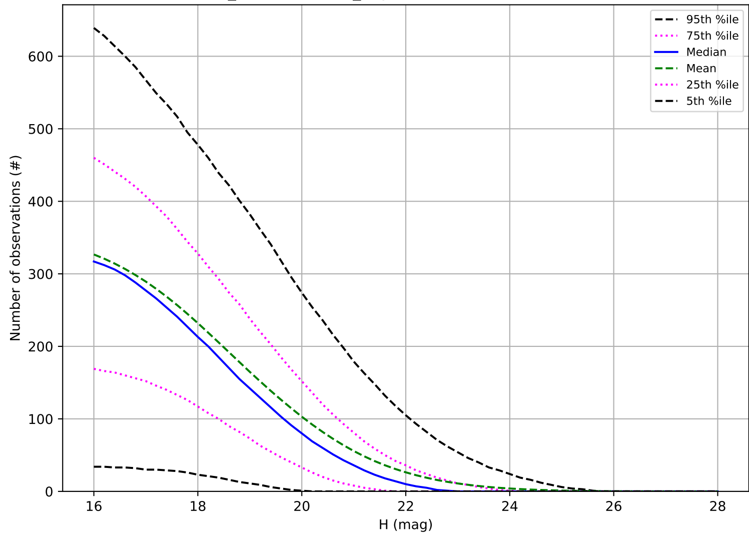
weather_cloudso14v3.4_10yrs: Number of observations NEO
