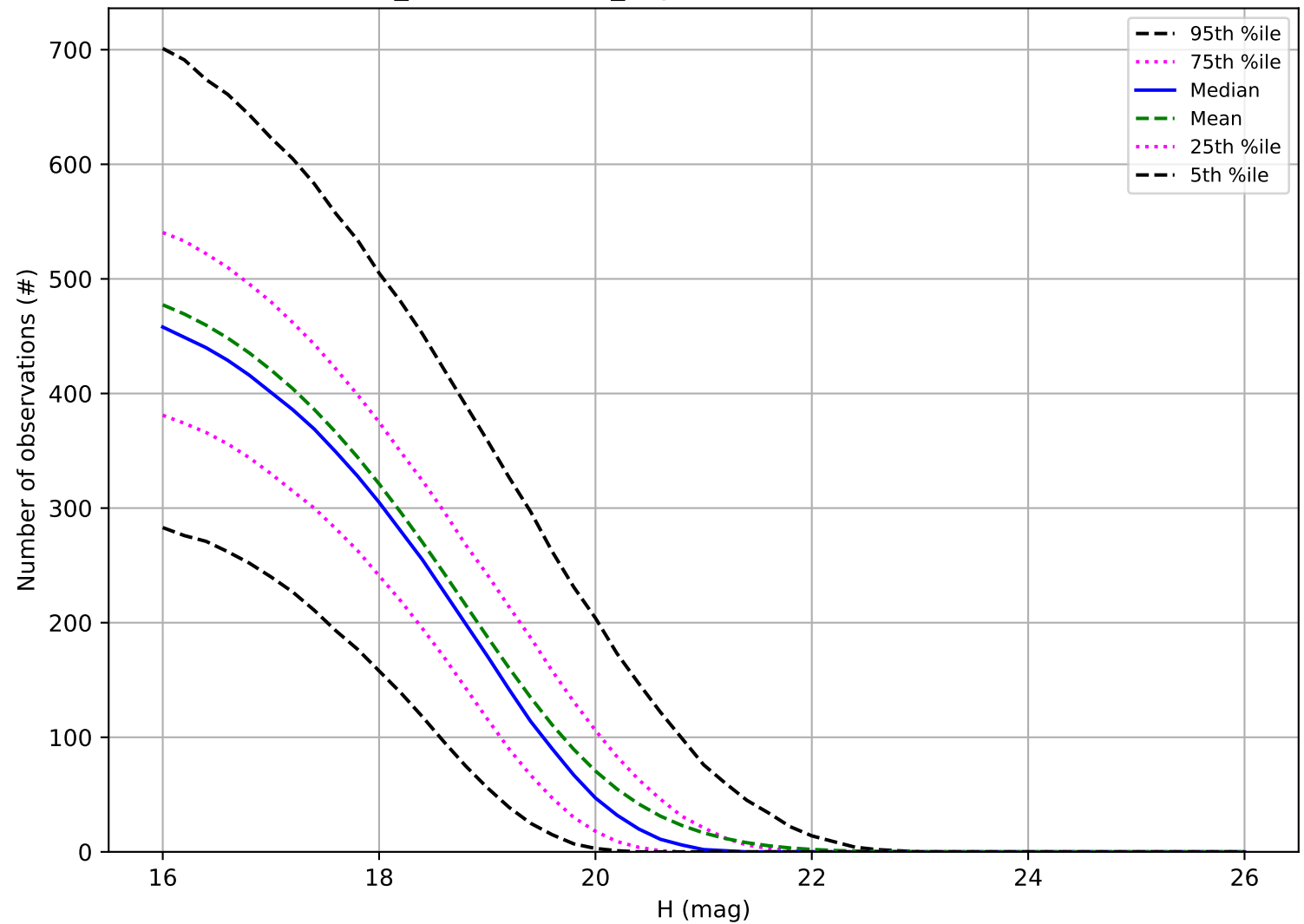
weather_cloudso14v3.4_10yrs: Number of observations MBA
