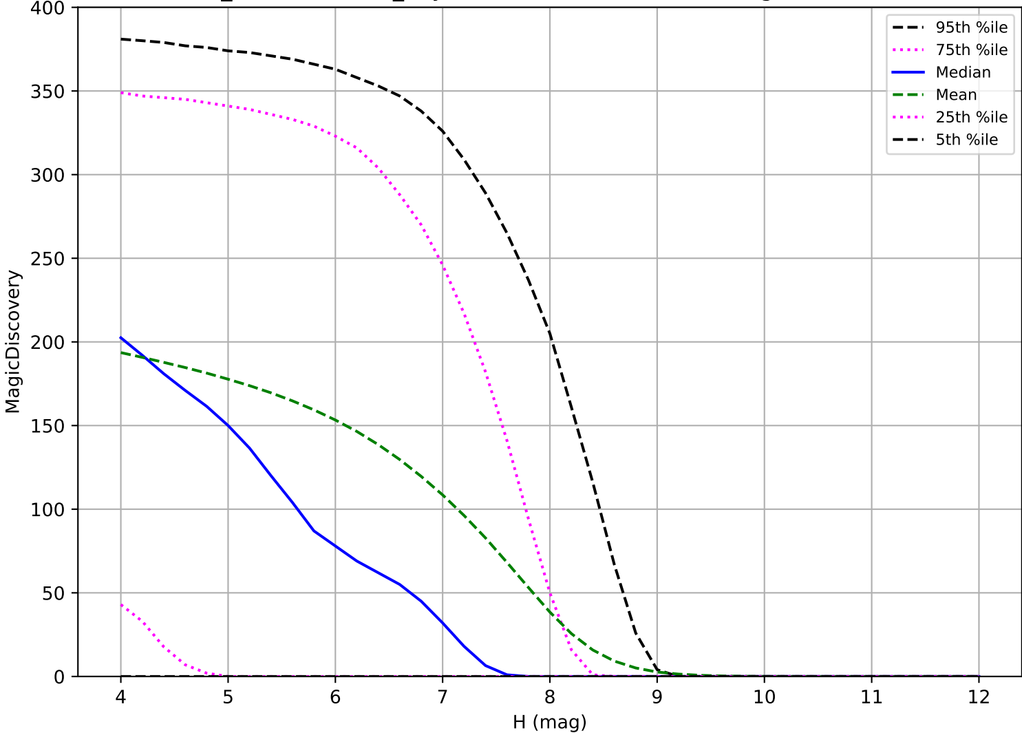
weather_cloudso14v3.4_10yrs: TNO 6 detections in 60 nights detection loss
