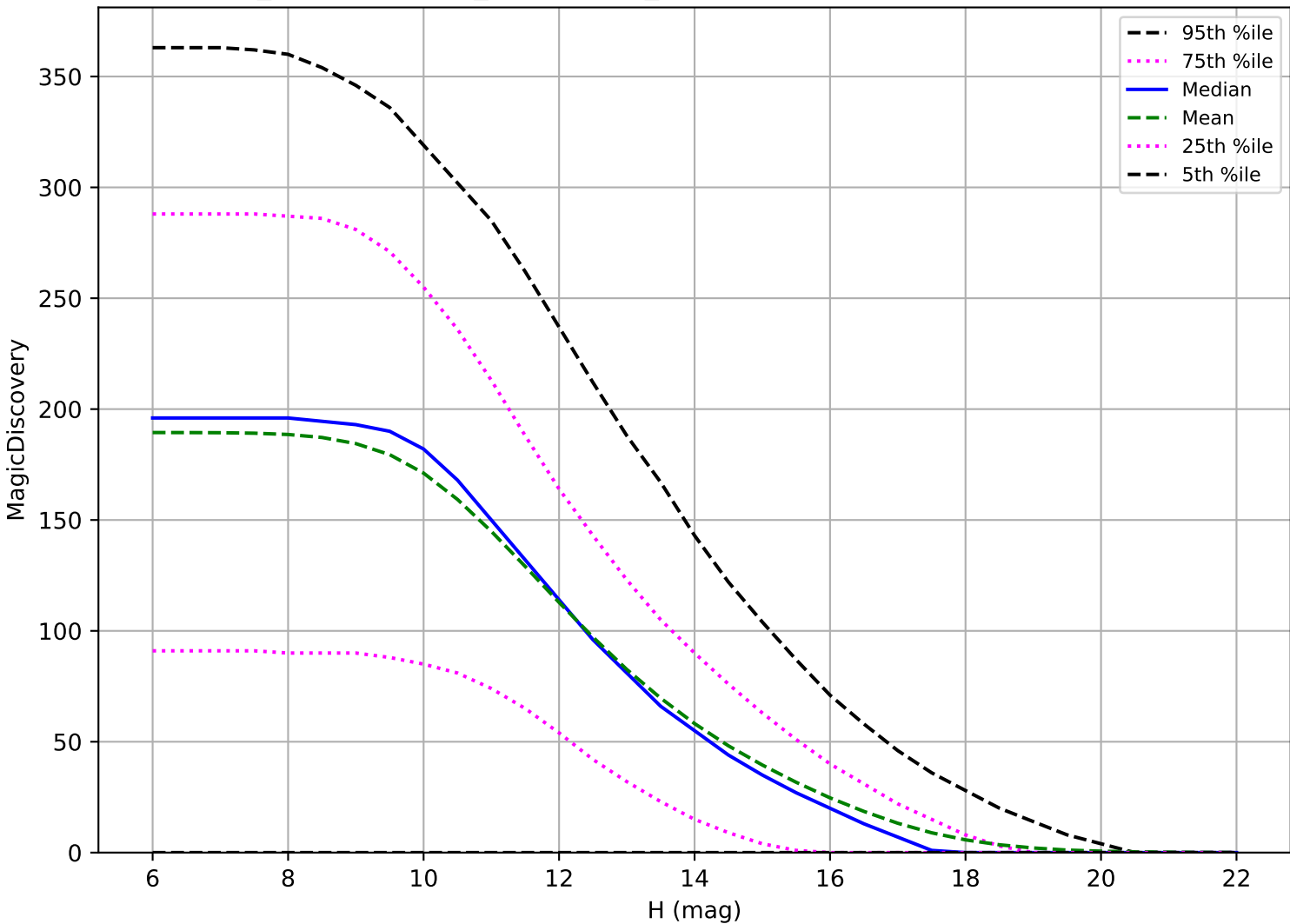
weather_cloudso14v3.4_10yrs: OCC_r5 6 detections in 60 nights detection loss
