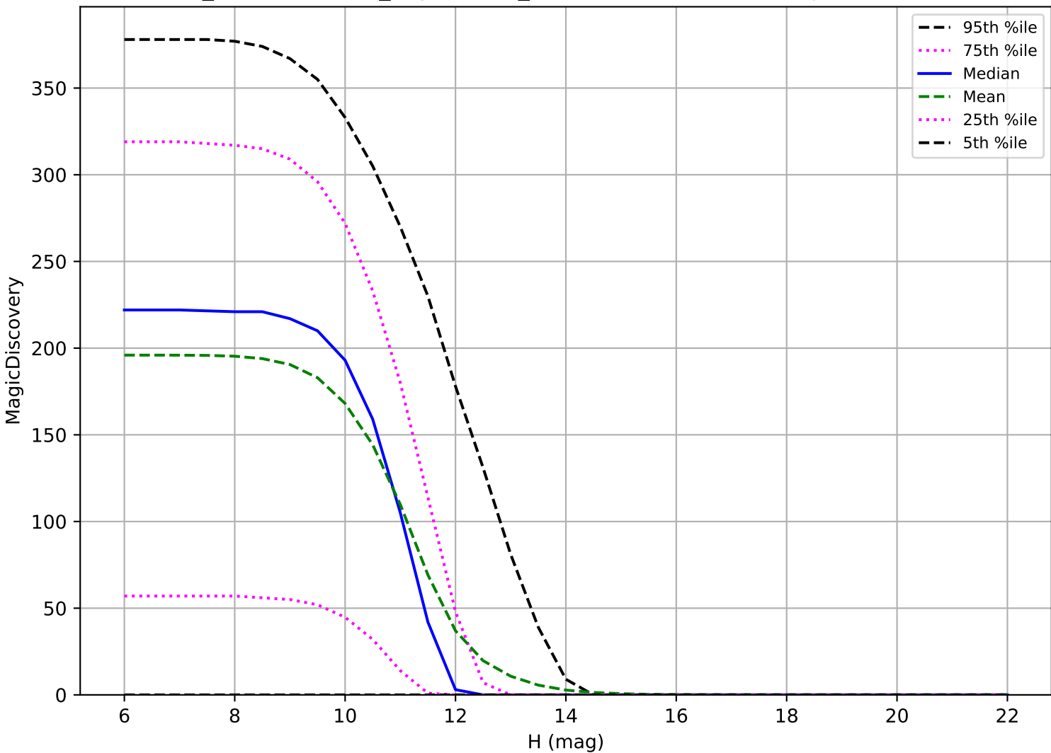
weather_cloudso14v3.4_10yrs: OCC_r20 6 detections in 60 nights detection loss
