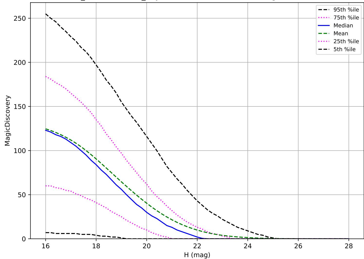
weather_cloudso14v3.4_10yrs: NEO 6 detections in 60 nights detection loss
