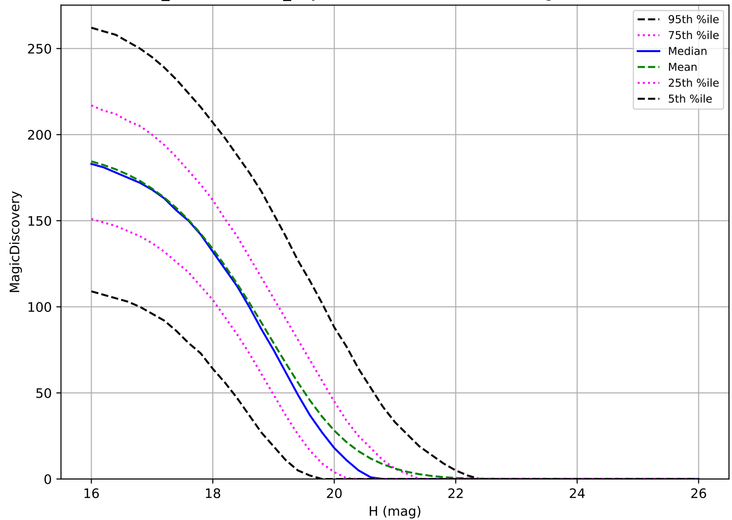
weather_cloudso14v3.4_10yrs: MBA 6 detections in 60 nights detection loss
