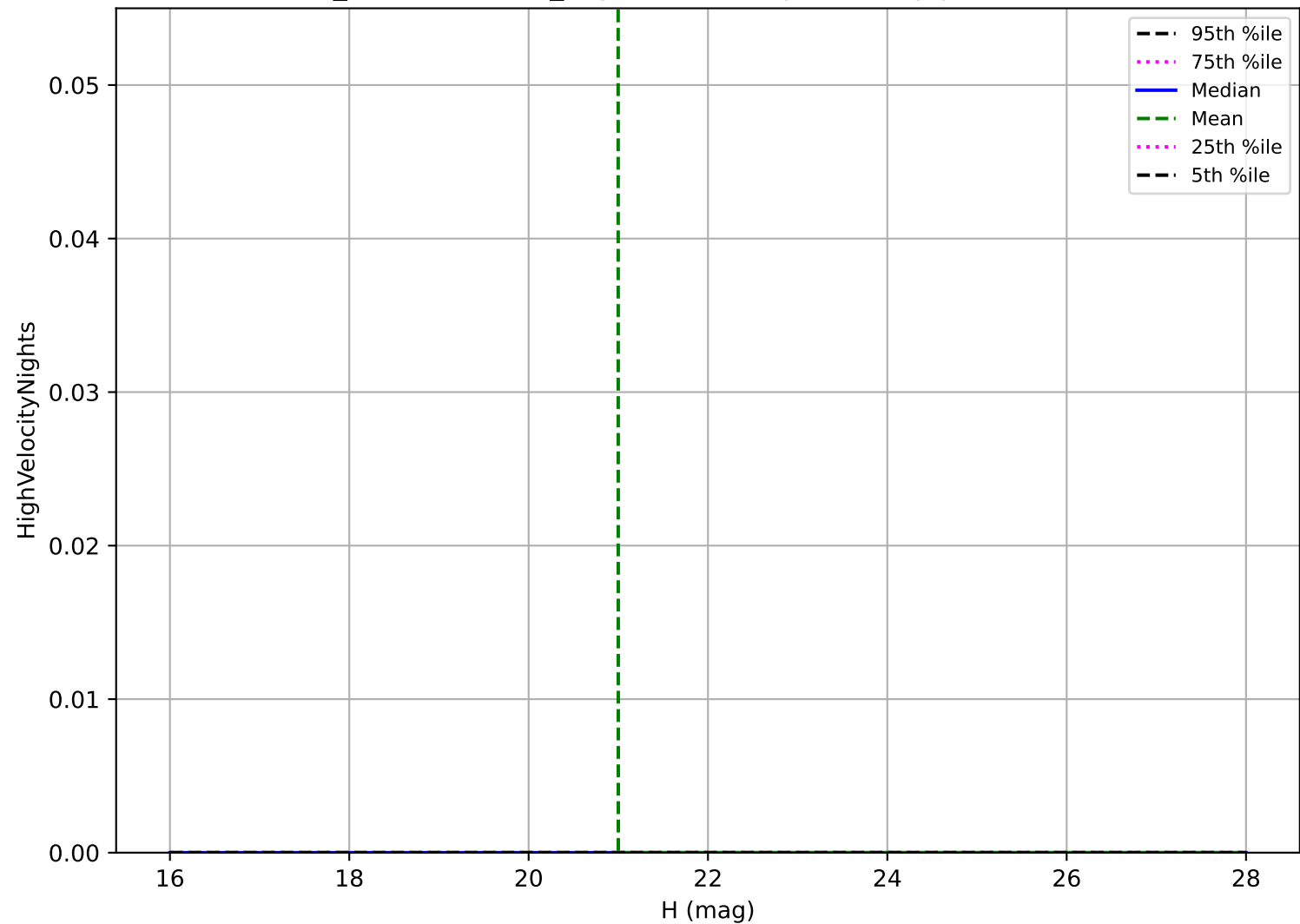
weather_cloudso14v3.4_10yrs: Vatira High velocity pair detection loss
