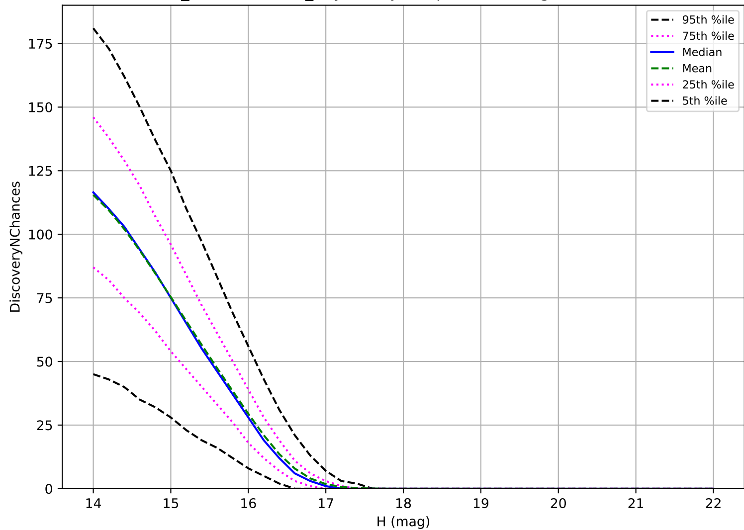
weather_cloudso14v3.4_10yrs: Trojan 3 pairs in 15 nights detection loss
