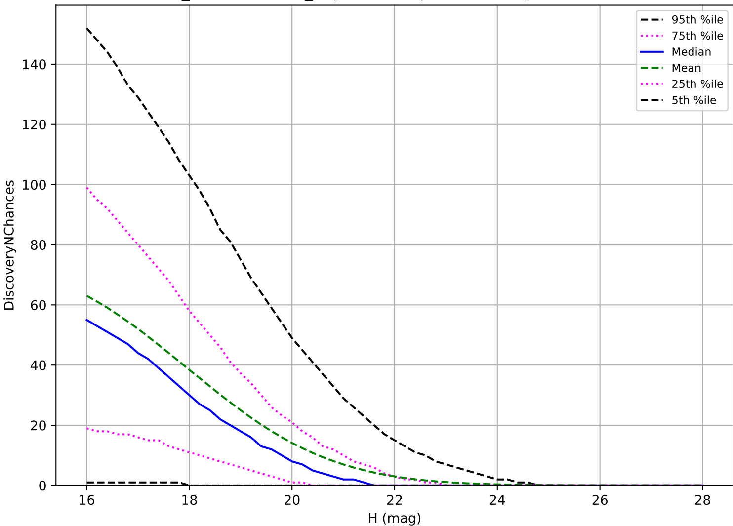
weather_cloudso14v3.4_10yrs: PHA 3 pairs in 15 nights detection loss
