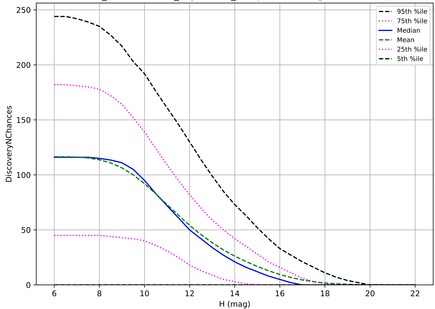
weather_cloudso14v3.4_10yrs: OCC_r5 3 pairs in 15 nights detection loss
