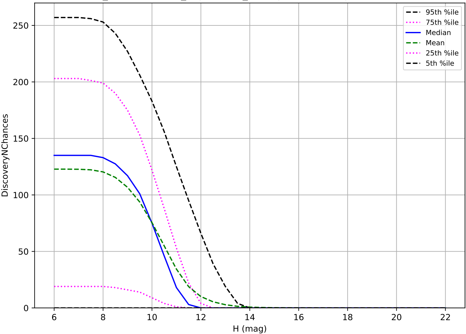
weather_cloudso14v3.4_10yrs: OCC_r20 3 pairs in 15 nights detection loss
