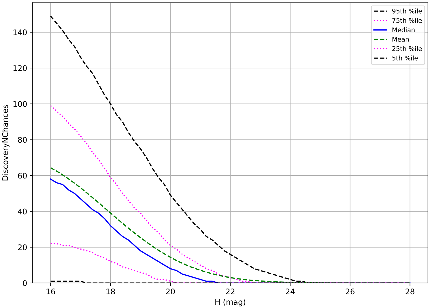
weather_cloudso14v3.4_10yrs: NEO 3 pairs in 15 nights detection loss
