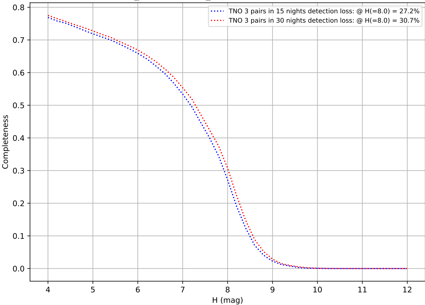
weather_cloudso14v3.4_10yrs: DifferentialCompleteness
