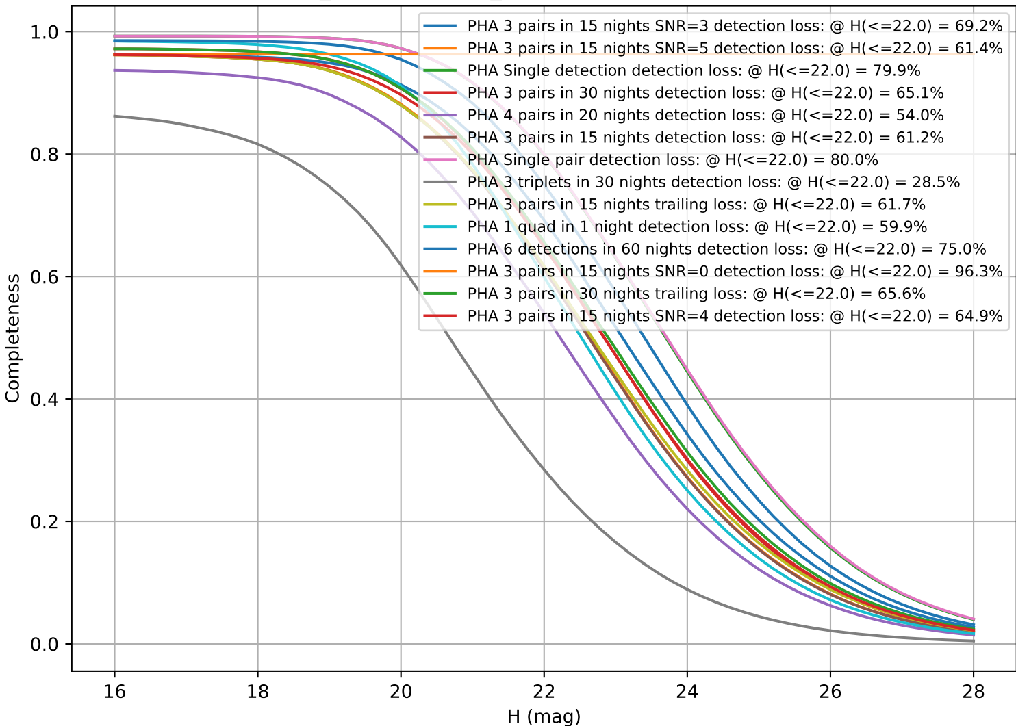
weather_cloudso14v3.4_10yrs: CumulativeCompleteness
