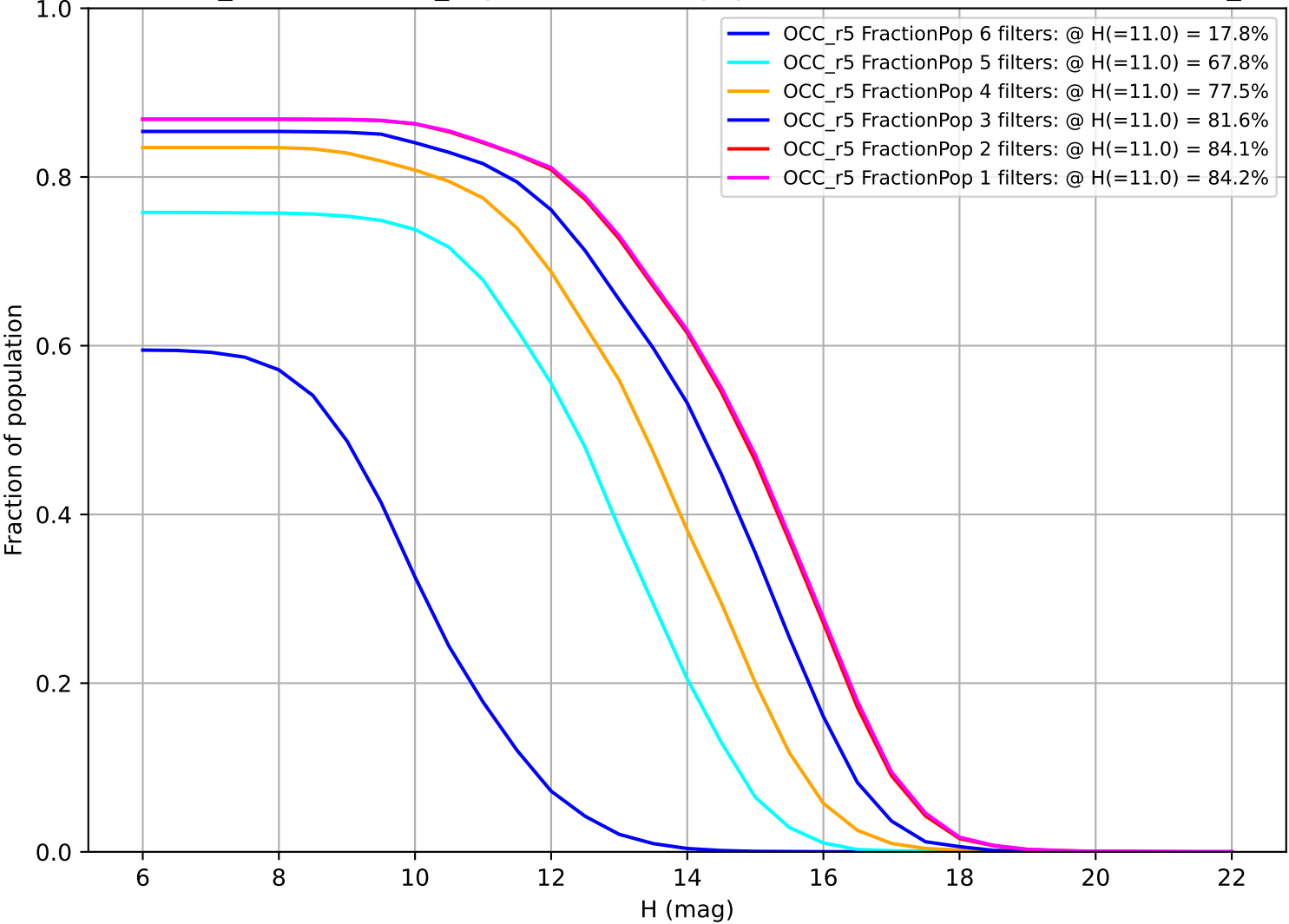
weather_cloudso14v3.4_10yrs: Fraction of population with colors in X filters OCC_r5
