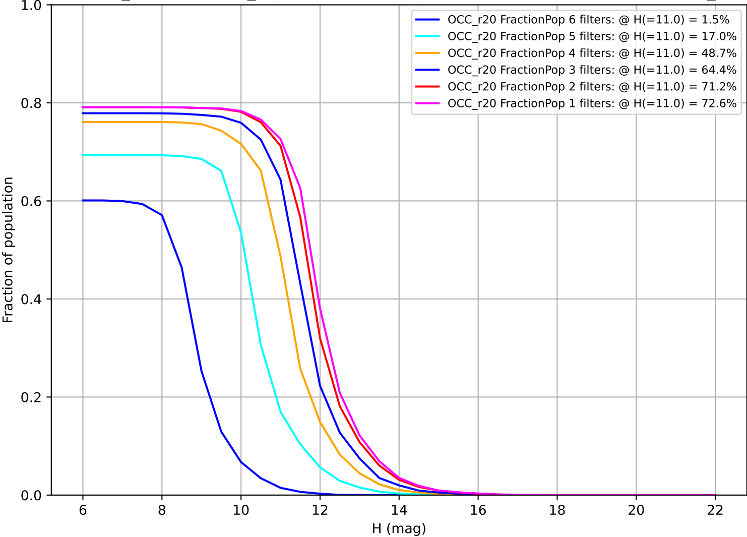
weather_cloudso14v3.4_10yrs: Fraction of population with colors in X filters OCC_r20
