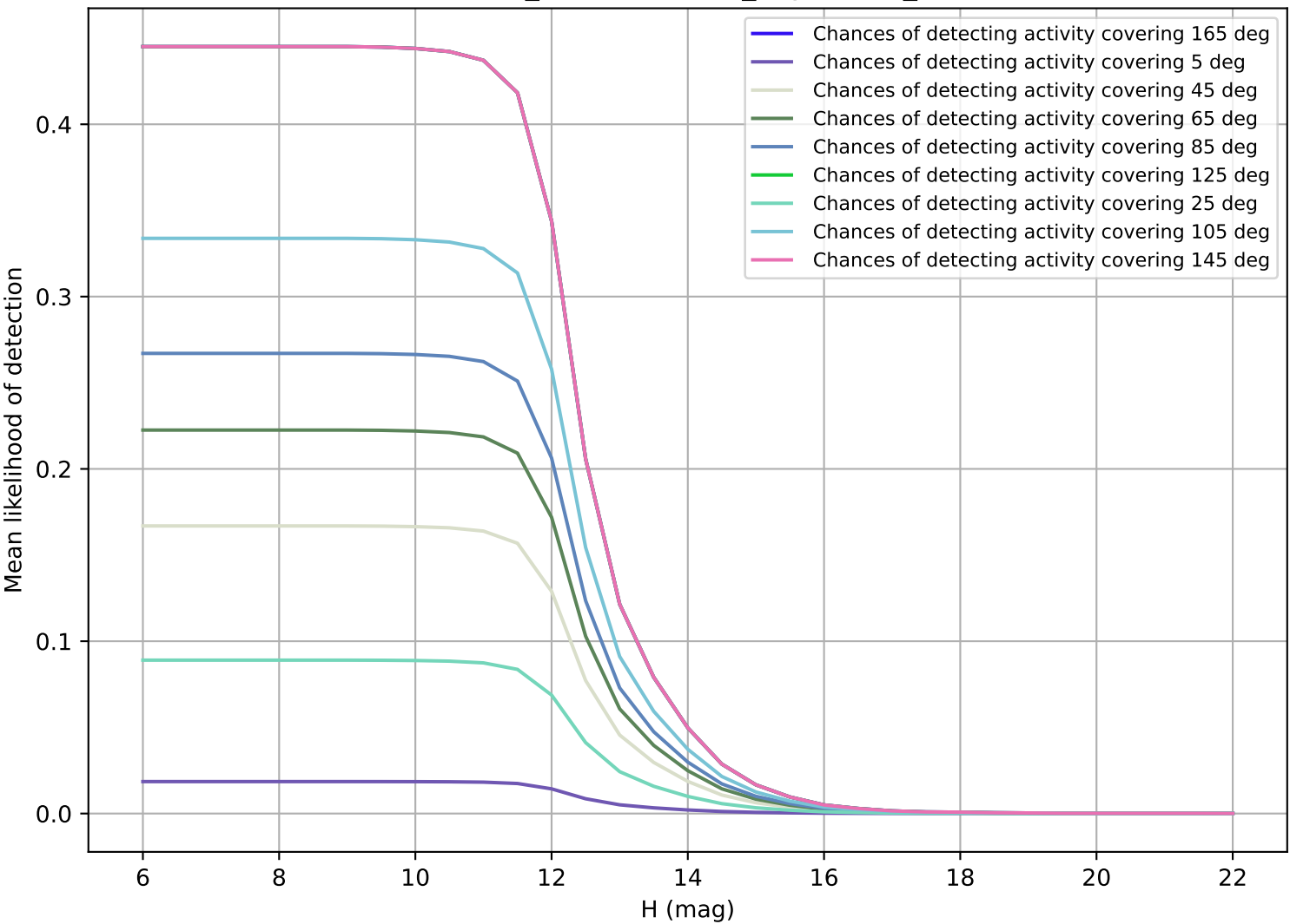
weather_cloudso14v3.4_10yrs OCC_r20
