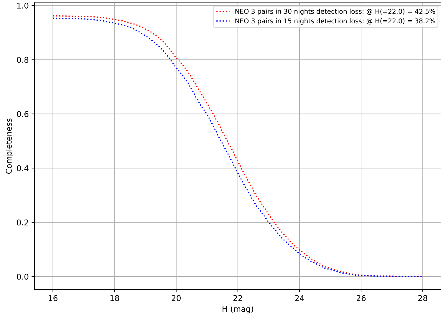
weather_cloudso14v3.4_10yrs: DifferentialCompleteness
