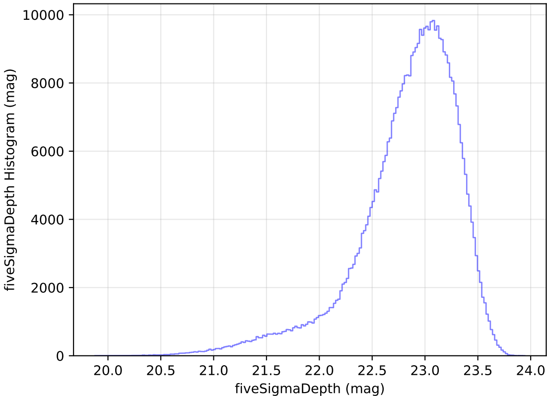
weather_cloudso14v3.4_10yrs z: fiveSigmaDepth Histogram
