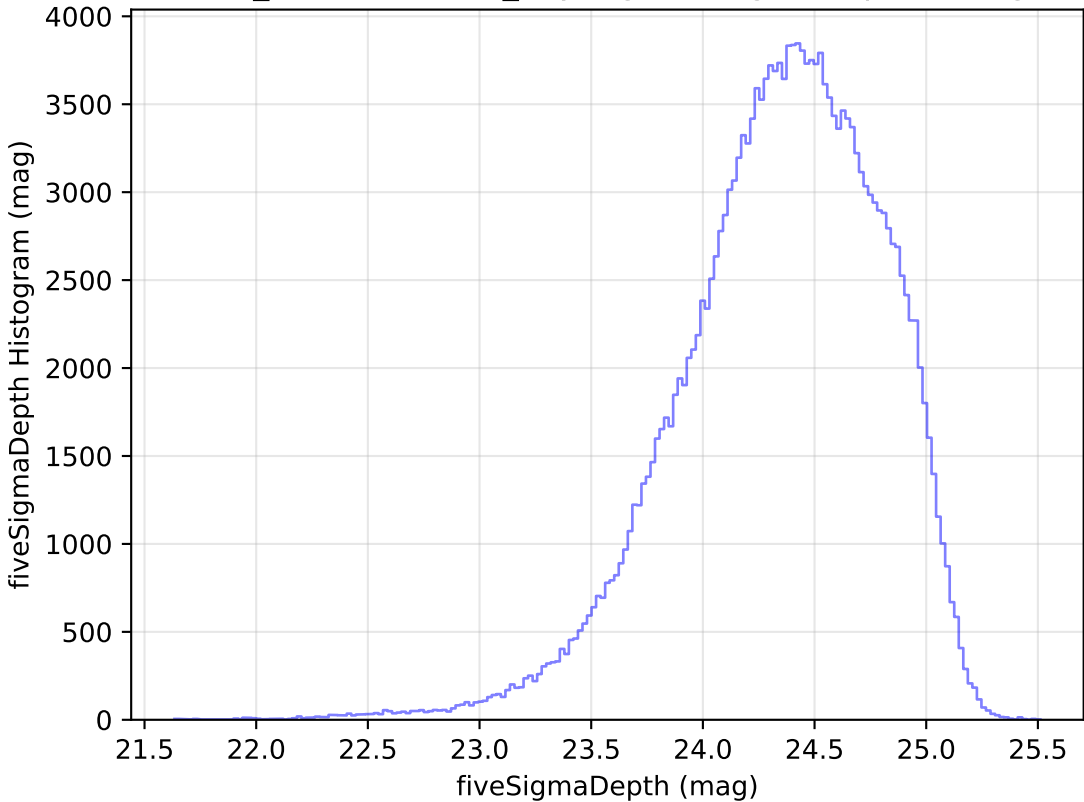
weather_cloudso14v3.4_10yrs g: fiveSigmaDepth Histogram
