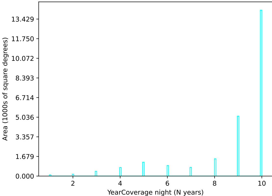
weather_cloudso14v3.4_10yrs u band: YearCoverage night
