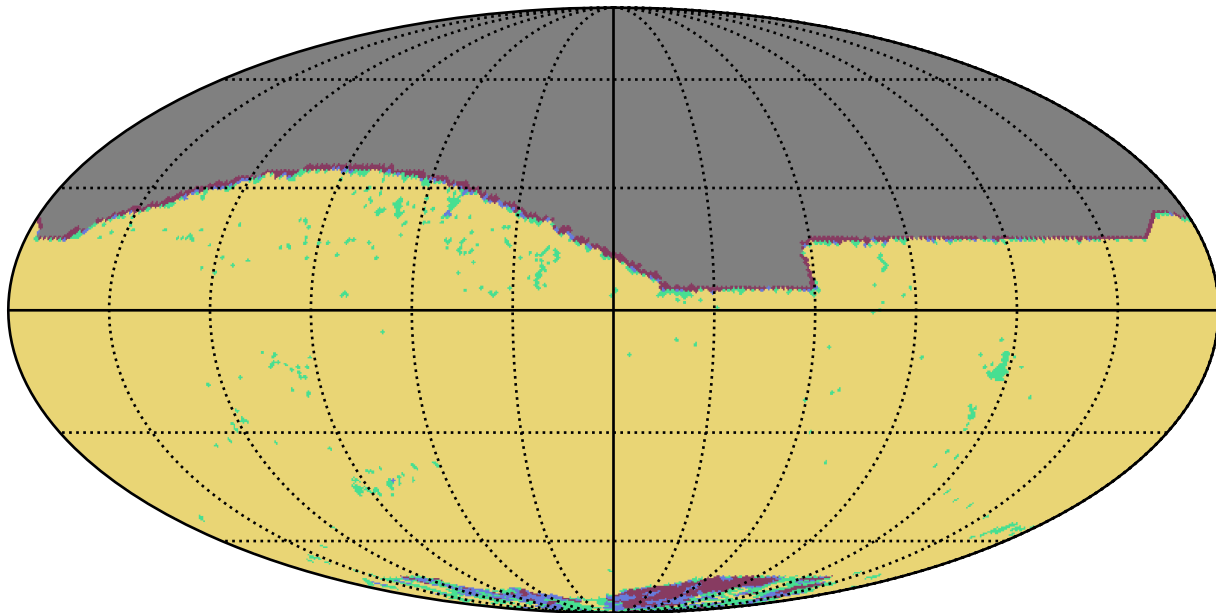
weather_cloudso14v3.4_10yrs r band: YearCoverage night
