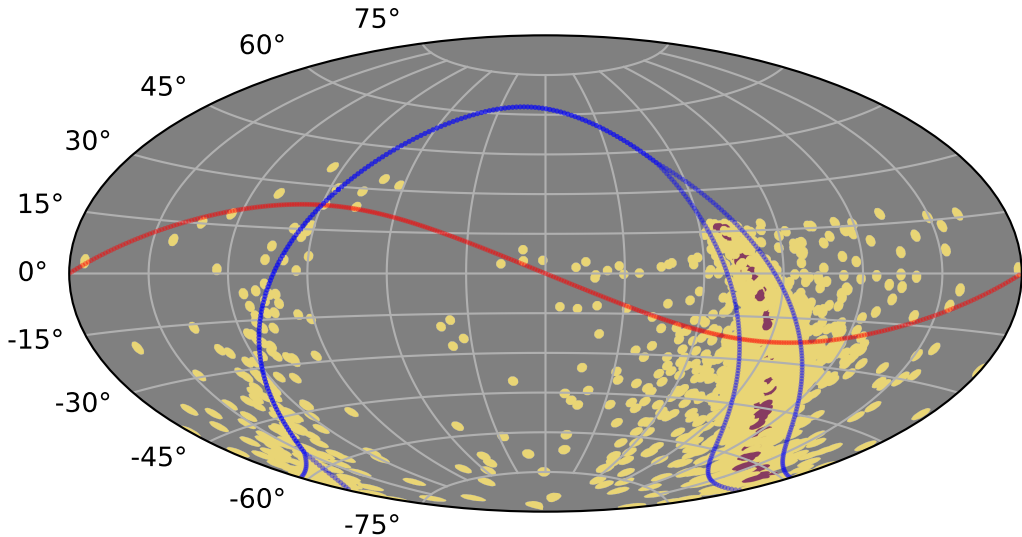
weather_cloudso14v3.4_10yrs : XRBPoMetric_possible_to_detect
