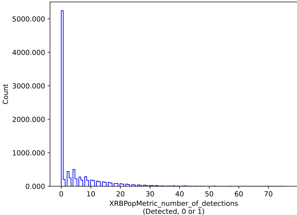
weather_cloudso14v3.4_10yrs : XRBPoMetric_number_of_detections
