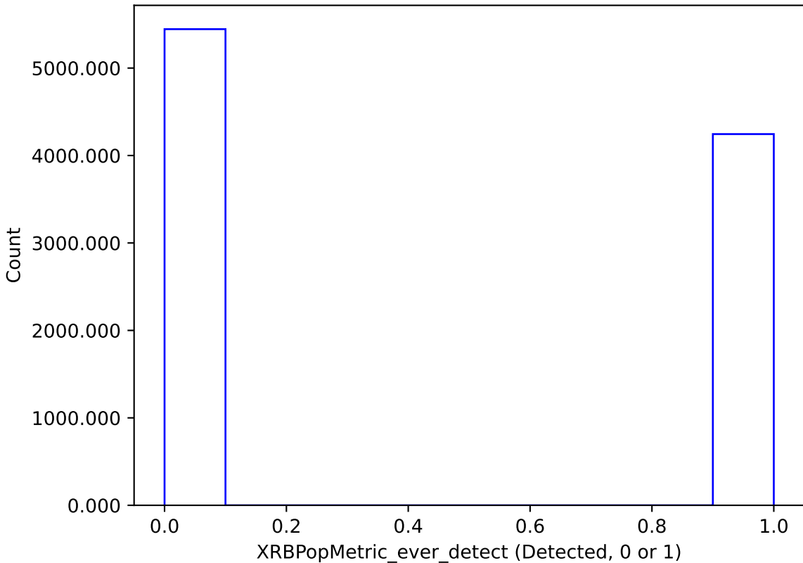
weather_cloudso14v3.4_10yrs : XRBPoMetric_ever_detect
