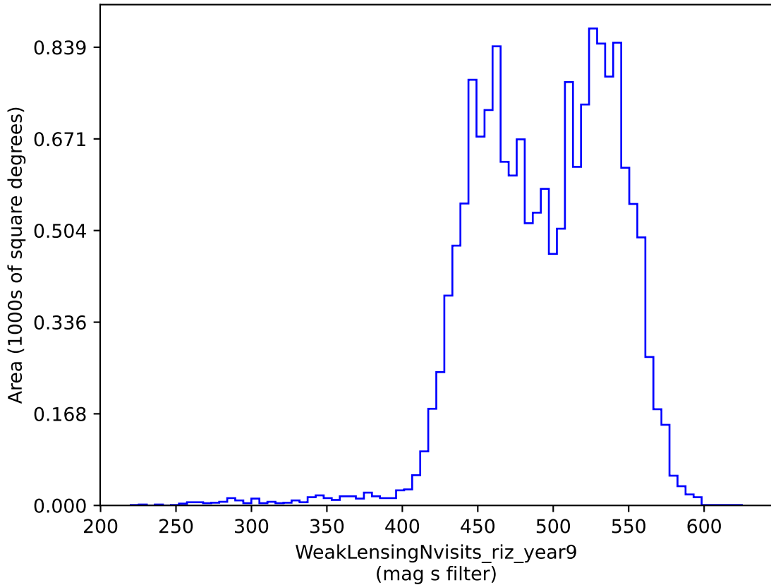
weather_cloudso14v3.4_10yrs gri band non-DD: WeakLensingNvisits_riz_year9
