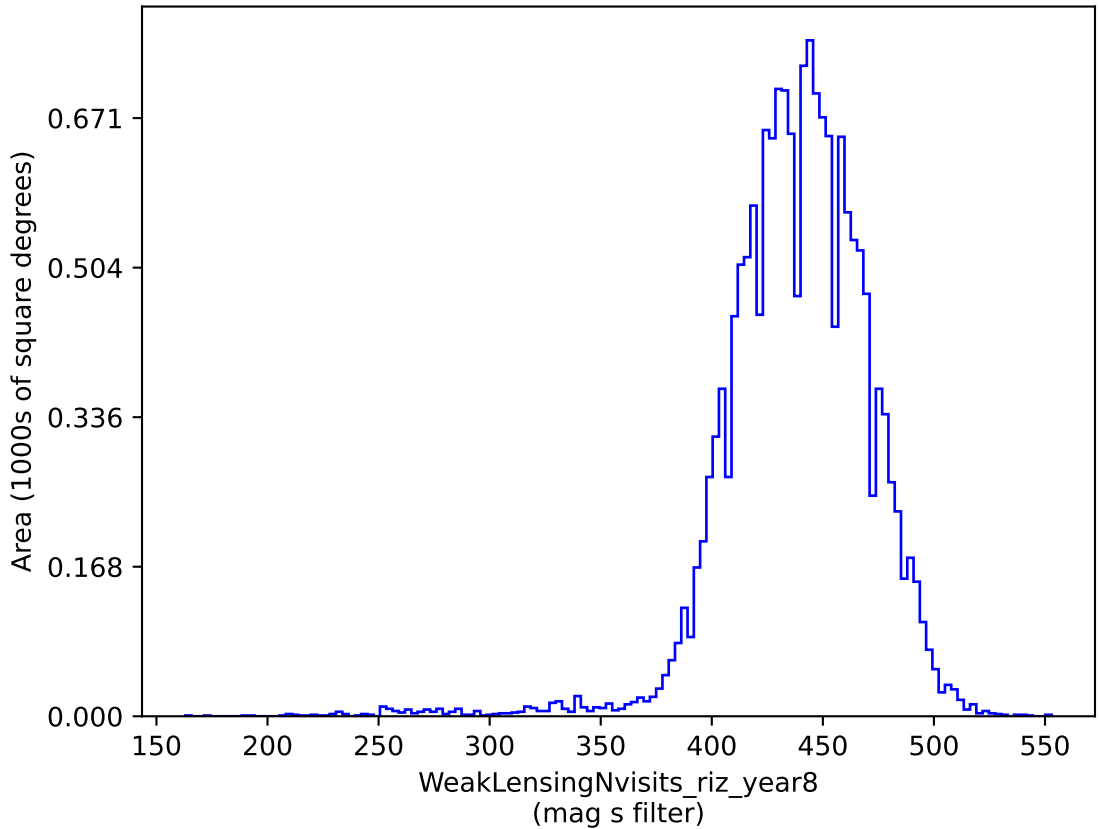
weather_cloudso14v3.4_10yrs gri band non-DD: WeakLensingNvisits_riz_year8
