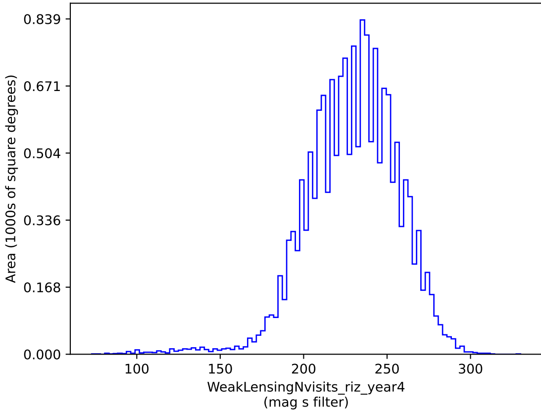
weather_cloudso14v3.4_10yrs gri band non-DD: WeakLensingNvisits_riz_year4
