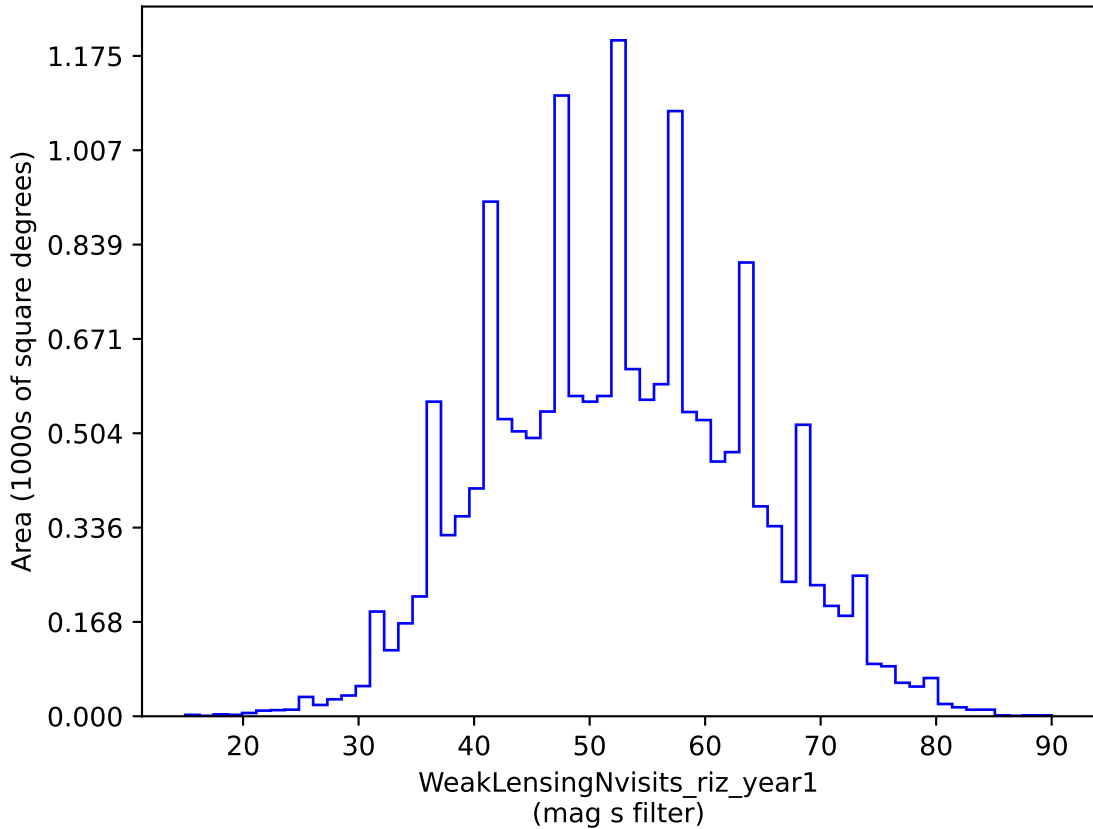
weather_cloudso14v3.4_10yrs gri band non-DD: WeakLensingNvisits_riz_year1
