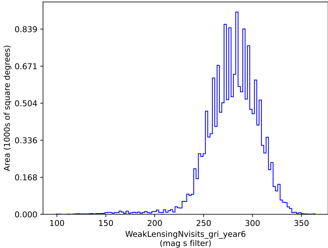
weather_cloudso14v3.4_10yrs gri band non-DD: WeakLensingNvisits_gri_year6
