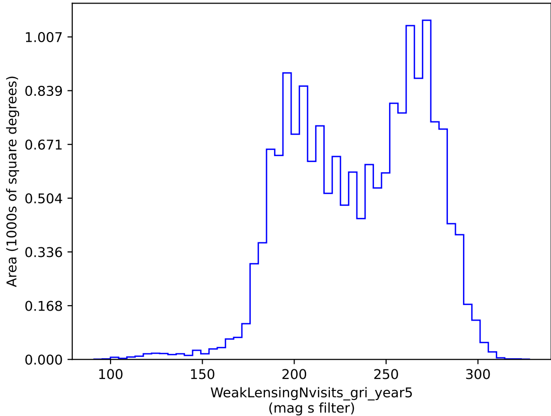
weather_cloudso14v3.4_10yrs gri band non-DD: WeakLensingNvisits_gri_year5
