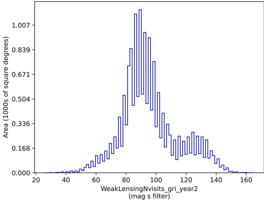
weather_cloudso14v3.4_10yrs gri band non-DD: WeakLensingNvisits_gri_year2
