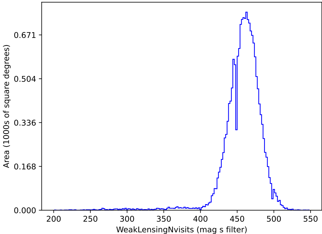
weather_cloudso14v3.4_10yrs gri band non-DD: WeakLensingNvisits
